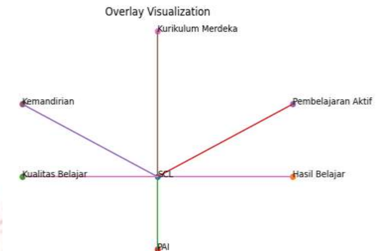
Gambar 1.3 Overlay Visualization
