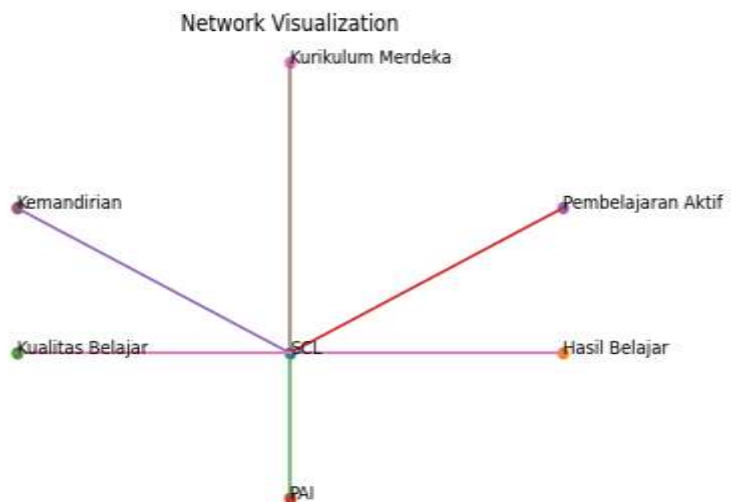
Gambar 1.2 Network Visualization
