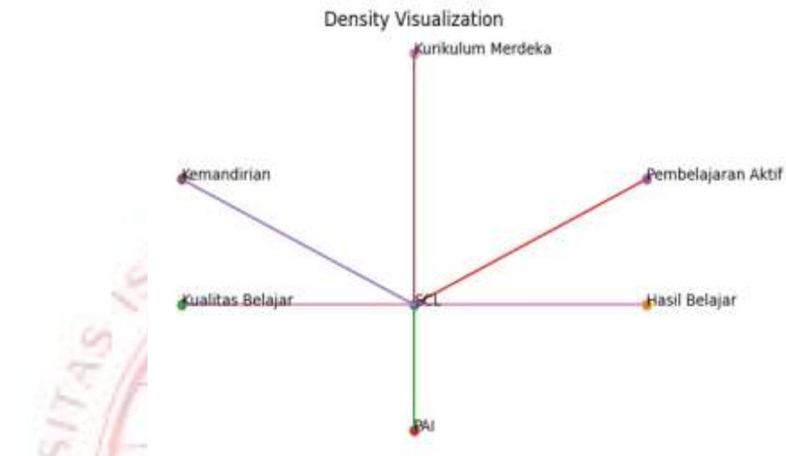
Gambar 1.4 DensityVisualization
